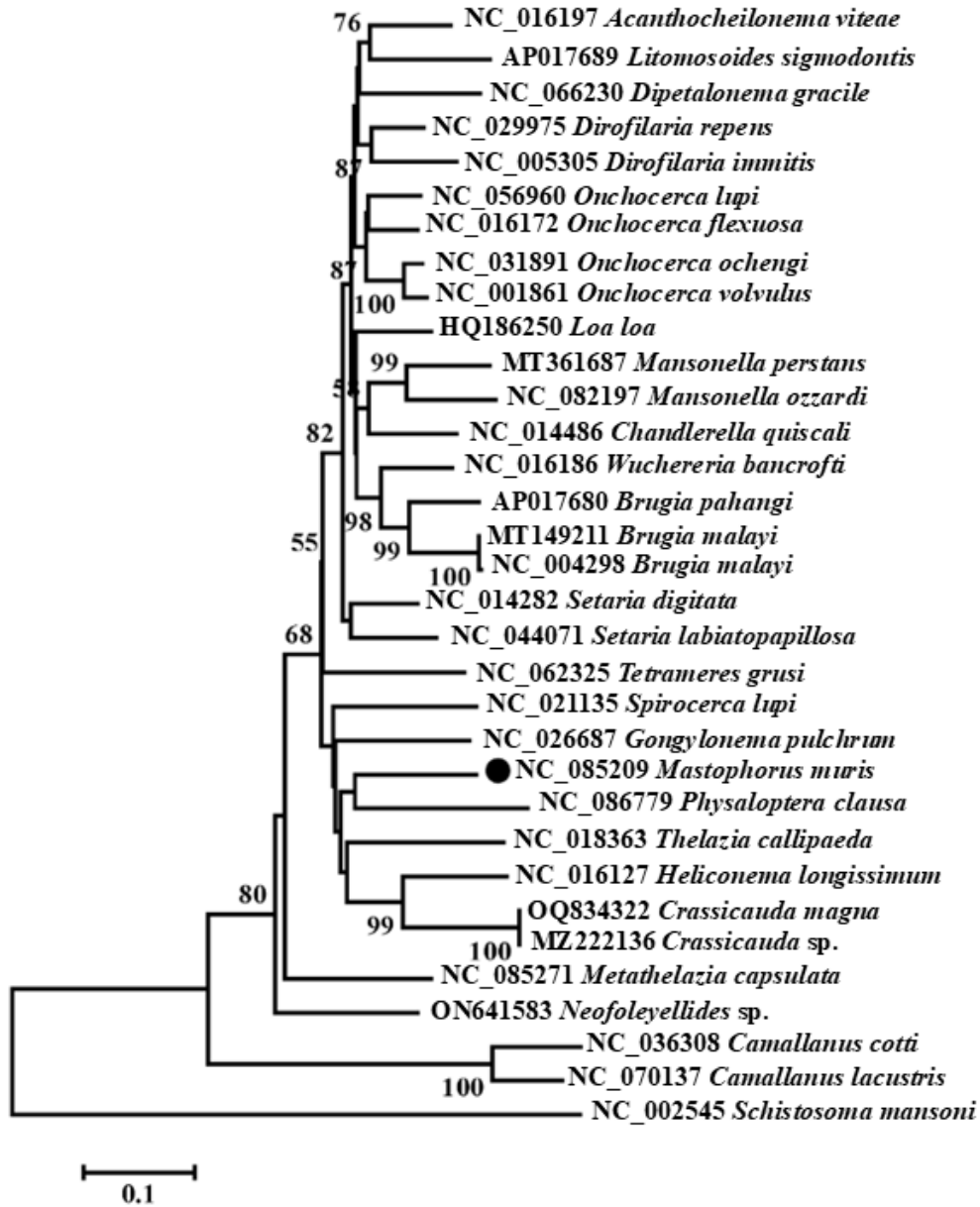
Fig. S11. Phylogenetic relationships among 30 species of selected Spiruromorpha nematodes inferred from Neighbor-Joining Method of nucleotide sequences of cytb genes. Schistosoma mansoni was used as the outgroup. Black dots represented Mastophorus muris .
