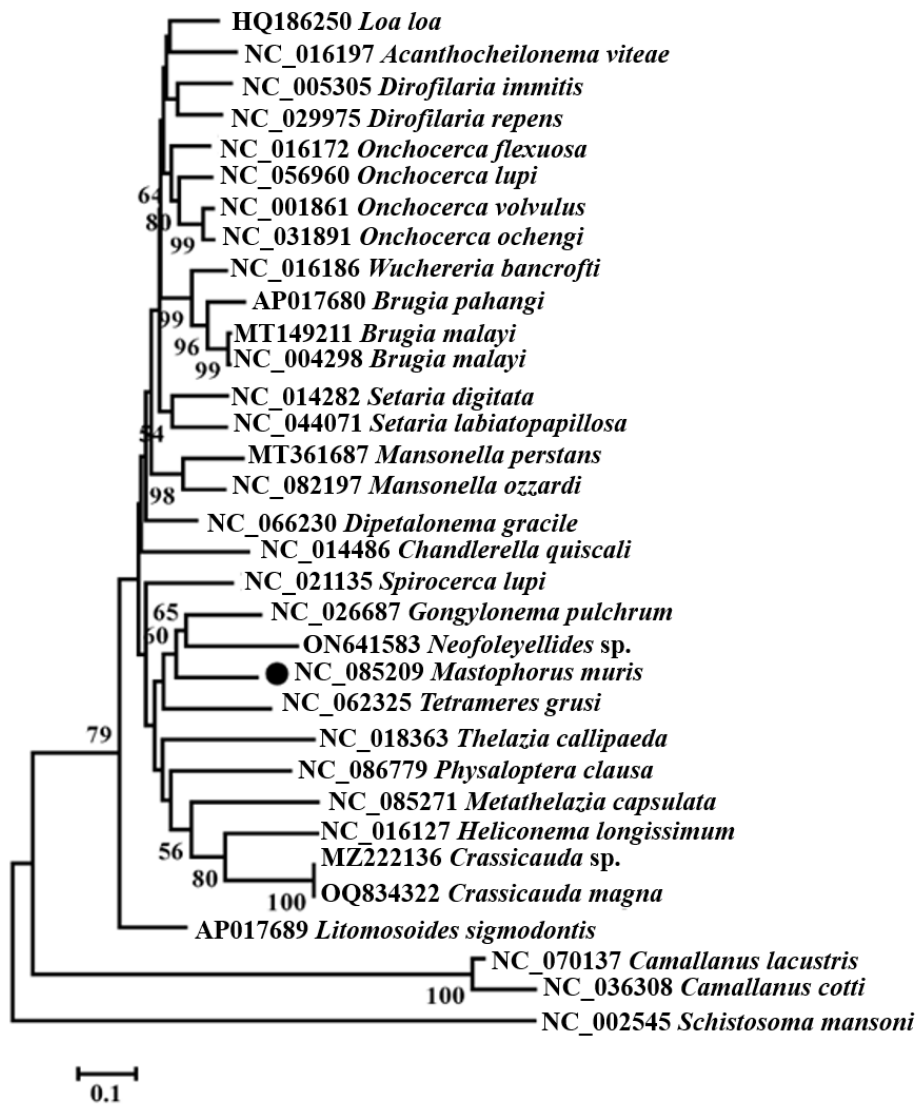
Fig. S12. Phylogenetic relationships among 30 species of selected Spiruromorpha nematodes inferred from Neighbor-Joining Method of nucleotide sequences of atp6 genes. Schistosoma mansoni was used as the outgroup. Black dots represented Mastophorus muris .
