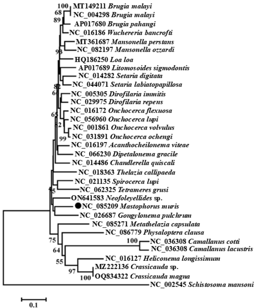
Fig. S13. Phylogenetic relationships among 30 species of selected Spiruromorpha nematodes inferred from Neighbor-Joining Method of nucleotide sequences of s-rRNA genes. Schistosoma mansoni was used as the outgroup. Black dots represented Mastophorus muris .
