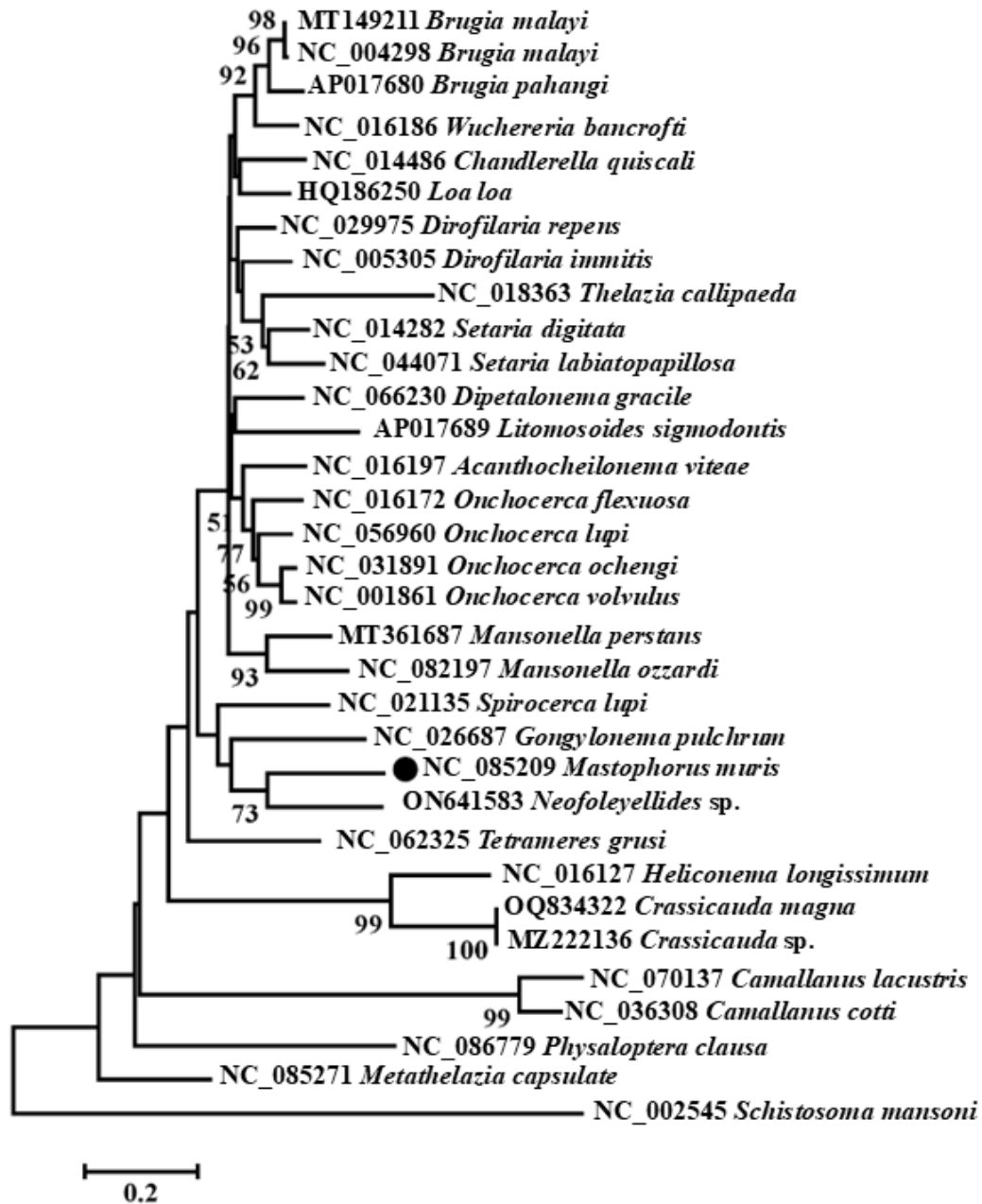
Fig. S9. Phylogenetic relationships among 30 species of selected Spiruromorpha nematodes inferred from Neighbor-Joining Method of nucleotide sequences of nad6 genes. Schistosoma mansoni was used as the outgroup. Black dots represented Mastophorus muris .
