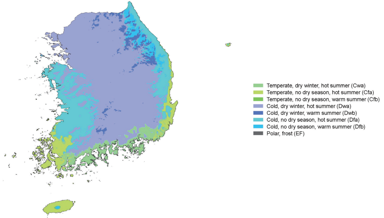
Supplementary Fig. S2. Köppen–Geiger climate classification maps for Korea (1980-2016) [18].
