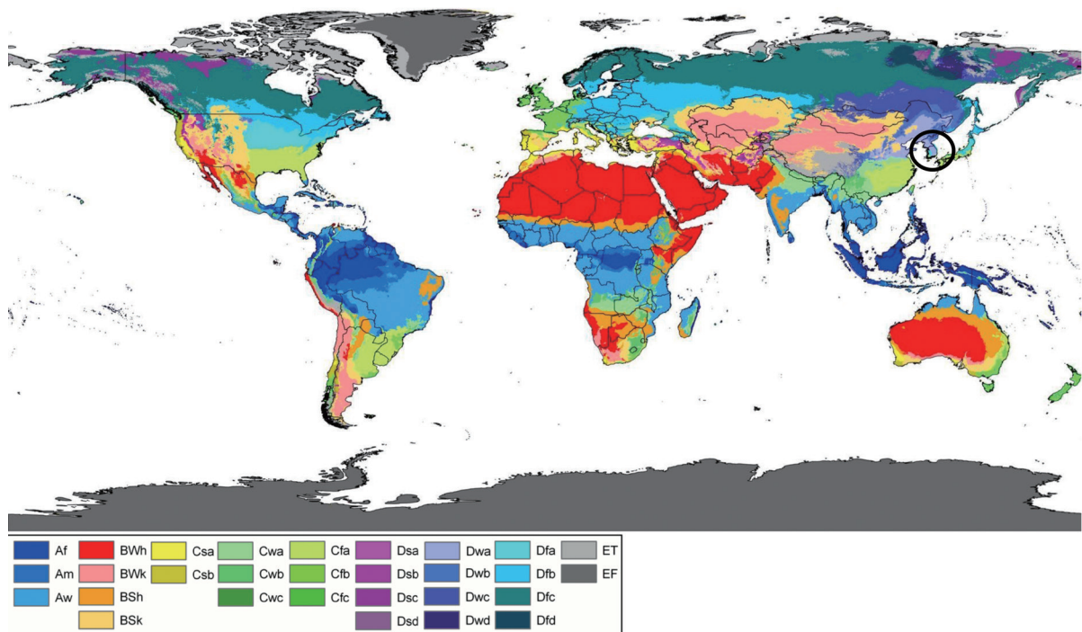
Supplementary Fig. S1. World climate distribution map based on the Köppen–Geiger classification (1980-2016). Af: equatorial climate; Am: monsoon climate; Aw: tropical savanna climate; BWh: warm desert climate; BWk: cold desert climate; BSh: warm semi-arid climate; BSk: cold semi-arid climate; Csa: warm mediterranean climate; Csb: temperate mediterranean climate; Cwa: humid subtropical climate; Cwb: humid subtropical climate/subtropical oceanic highland climate; Cwc: oceanic subpolar climate; Cfa: warm oceanic climate/humid subtropical climate; Cfb: temperate oceanic climate; Cfc: cool oceanic climate; Dsa: warm continental climate/mediterranean continental climate; Dsb: temperate continental climate/mediterranean continental climate; Dsc: cool continental climate; Dsd: cold continental climate; Dwa: warm continental climate/humid continental climate; Dwb: temperate continental climate/humid continental climate; Dwc: cool continental climate/subarctic climate; Dwd: cold continental climate/subarctic climate; Dfa: warm continental climate/humid continental climate; Dfb: temperate continental climate/humid continental climate; Dfc: cool continental climate/subarctic climate; Dfd: cold continental climate/subarctic climate; ET: tundra climate; EF: ice cap climate [18].
